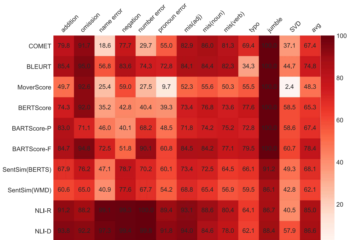
Figure 1: Average accuracy (values in each block) of all metrics per phenomenon over the adversarial datasets for ref-based MT evaluation. Darker color indicates higher accuracy and vice versa.
