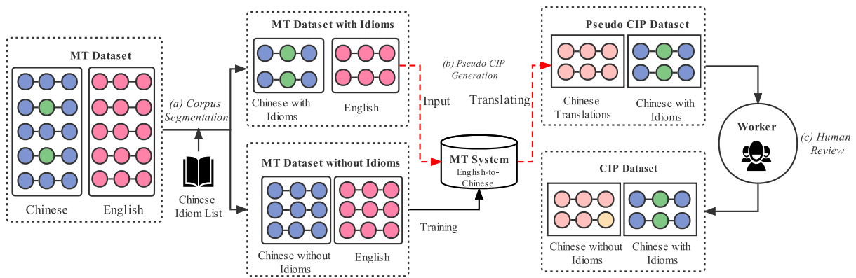
Figure 2: A pipelined illustration of creating a CIP dataset based on a Chinese-English MT corpus. (a) The corpus is split into an idiom-containing sub-corpus and a non-idiom-containing sub-corpus based on a Chinese idiom list. (b) We train a MT system using the non-idiom-containing sub-corpus, and create a pseudo-CIP Dataset by pairing the original Chinese idiom-containing sentences and the translated non-idiom-containing sentences using the trained MT system. (c) We ask human annotators to revise the translated Chinese sentence of the pairs to strengthen the quality of the created CIP dataset.
