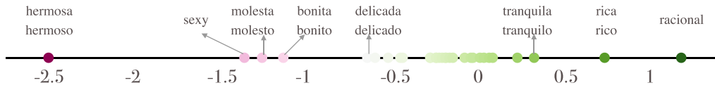
Figure 6: \psi_{\text{paired}}^{(a)} values computed using Equation (14) to measure causal gender bias in masked adjective prediction.
