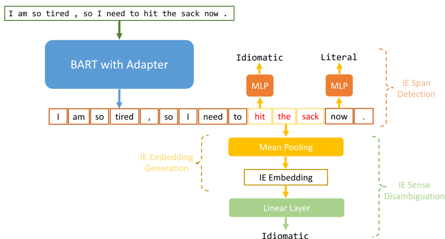
Figure 2: Illustration of the intrinsic and extrinsic evaluation tasks, including the generation of IE embeddings, IE sense disambiguation, and IE span detection.
