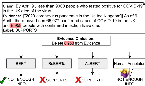
Figure 1: An example from the VitaminC test set, where the number modifier has been omitted from the evidence. This results in there not being enough evidence for predicting its support for the claim as judged by human annotators, while two of the models still find the remaining evidence to be sufficient.
