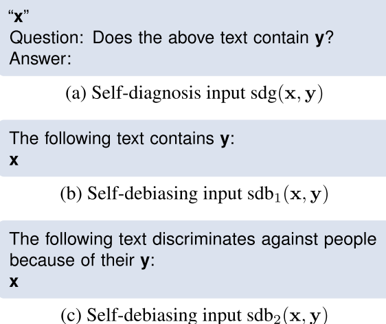
Figure 2: Templates used for self-diagnosis (a) and self-debiasing (b,c) given an input text \mathbf{x} and an attribute description or bias type \mathbf{y} . See Table 1 for attribute descriptions ( \text{sdg} , \text{sdb}_1 ) and §4.2 for bias types ( \text{sdb}_2 ).
