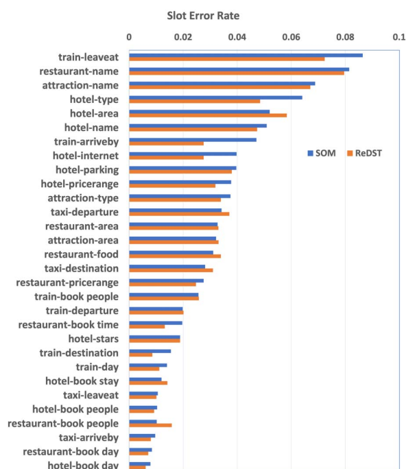
Figure 3: Slot error rate on the test set. The error rate for name slots on restaurant , hotel , and attraction domain drops 4.2% on average.
