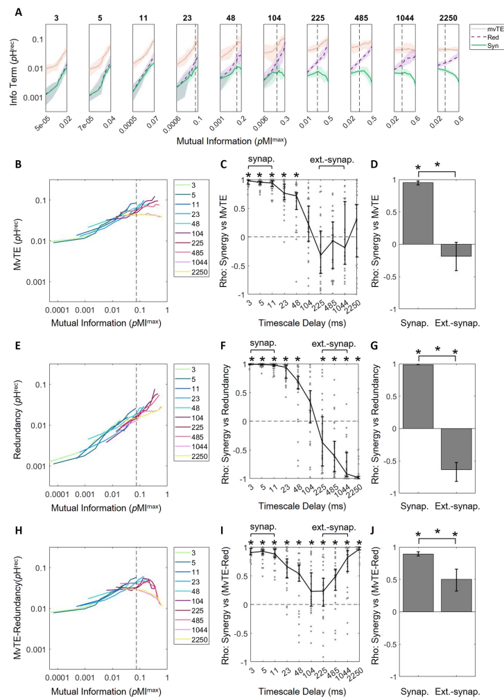
Figure 5. Redundancy encroaches upon multivariate transfer entropy at longer timescales, accounting for decreasing synergy at those timescales. (A) Log-scaled multivariate transfer entropy (mvTE), redundancy (Red), and synergy (Syn) versus mutual information, for all timescales. Growth of mvTE with respect to mutual information is steep at short timescales, but decreases across timescales. Redundancy grows with mutual information at all timescales. (B) MvTE curves in A plotted on the same axes. (C) Spearman rank correlation coefficients of synergy versus mvTE across timescales indicates that mvTE saturates at longer timescales. (D) Synergy and mvTE are significantly positively related at synaptic timescales, but not at extrasynaptic timescales. (E) Redundancy curves in A plotted on the same axes. (F) Spearman rank correlation coefficients of synergy versus redundancy across timescales shows how the two are positively related at shorter timescales and negatively related at longer timescales. (G) Synergy and redundancy are significantly positively related at synaptic timescales and significantly negatively related at extrasynaptic timescales. (H) Difference of MvTE and redundancy curves in A plotted on the same axes shows that the overall trend looks most similar to that of synergy versus mutual information in Figure 4E. (I) Spearman rank correlation coefficients of synergy versus mvTE redundancy across timescales shows that the two are positively related at all timescales. (J) Synergy and mvTE redundancy are significantly positively related at synaptic and extrasynaptic timescales. Synergy versus mutual information data has been replotted from Figure 4D here in A for ease of comparison. For all plots, solid/bold lines indicate medians and shaded regions/error bars depict 95% bootstrap confidence intervals around the median.
