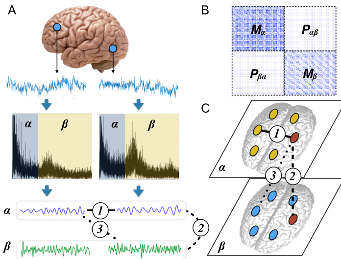
Figure 1. Encoding brain dynamics as a multilayer functional network. We show an illustrative example with two frequency bands (alpha and beta). (A) We band-pass filter the MEG signals at two frequency bands: alpha [8–12] Hz and beta [12–30] Hz. We use mutual information (MI; MacKay, 2003) to quantify coordination between brain regions. This yields three different type of functional edges: Edge type “1” quantifies coordination between different regions at the same frequency band; edge type “2” corresponds to interlayer edges, which couple the activity of the same region at different frequency bands; and edge type “3” quantifies cross-frequency coupling (CFC) between two brain regions. Multiplex networks include only edges of types 1 and 2, whereas more general multilayer networks include all three types of edges. (B) Schematic of the supra-adjacency matrix of a two-layer network constructed from the data in panel A. (C) Schematic of the intralayer and interlayer edges in the multilayer functional network.
