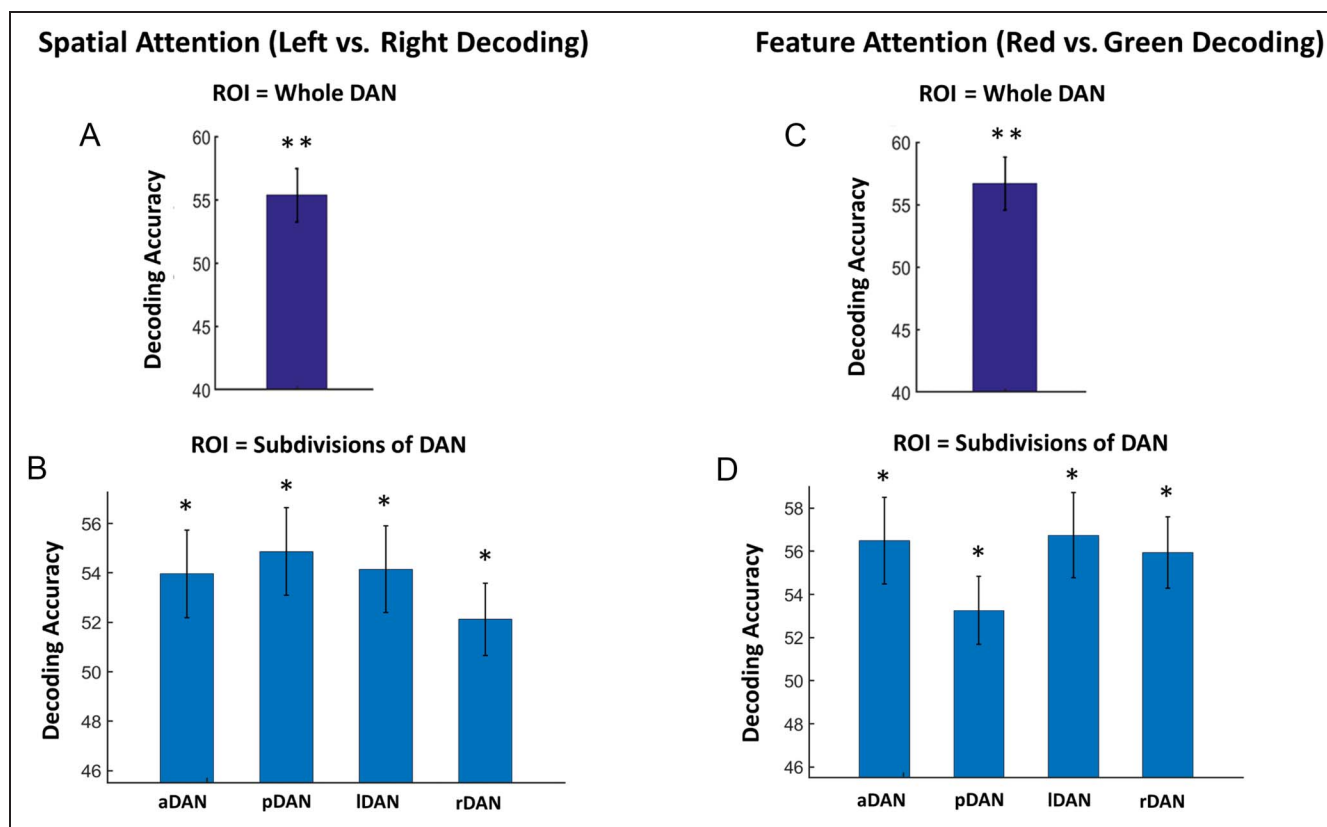
Figure 4. MVPA decoding accuracy for preparatory spatial and feature attention. Cue-evoked BOLD activation was estimated on a trial-by-trial basis. SVM was applied to decode different attention control conditions. Decoding accuracy for spatial attention (attend left vs. attend right): (A) within DAN as a whole and (B) within subdivisions of DAN. Decoding accuracy for color attention (attend red vs. attend green): (C) within DAN as a whole and (D) within subdivisions of DAN (** p < .0001 , * p < .05 ).
