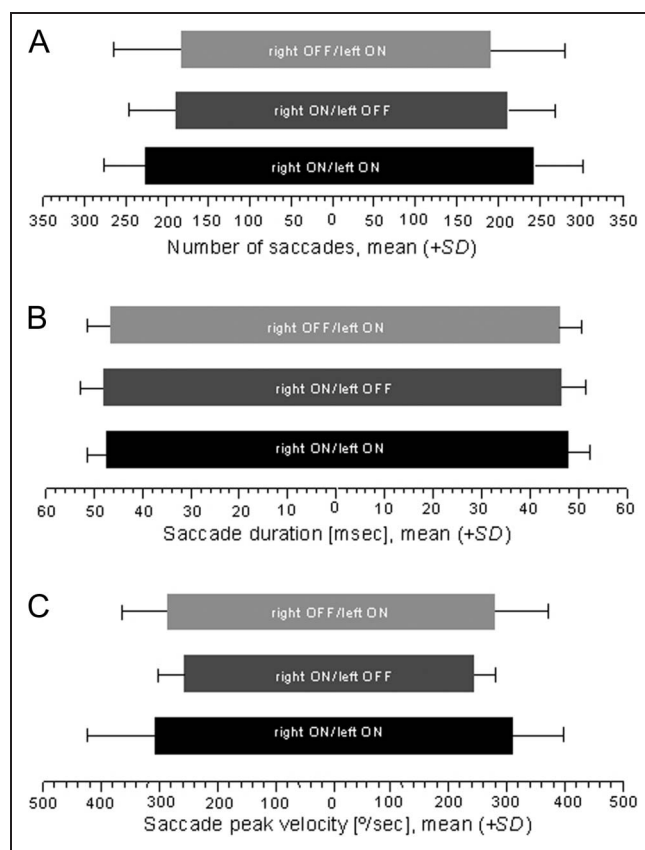
Figure 4. Saccade parameters are shown for right- and left-sided saccades: (A) number of saccades, (B) saccade duration, and (C) peak velocity. Data are given in mean ( \pm SD).
