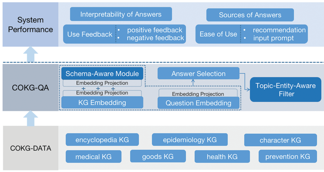
Figure 1. Architecture of the COKG-QA system.
