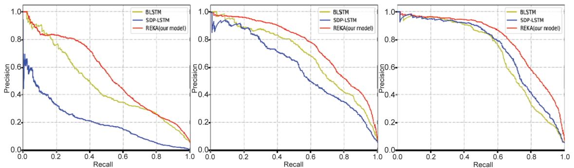
Figure 5. Precision-Recall curves of different used numbers of datasets (1%, 20%, 100%, respectively) and compared with RNN methods.
