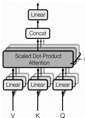
Figure 2. A sample of Multi-Head Attention [17]
