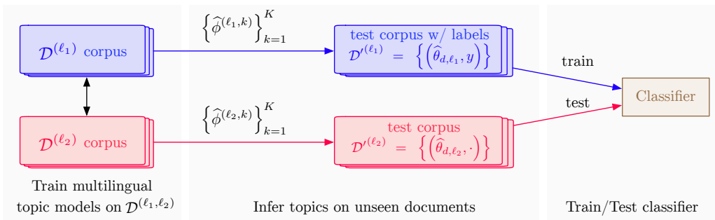
Figure 11 An illustration of crosslingual document classification. After training multilingual topic models, the topics, \{\hat{\phi}^{(\ell, k)}\} are used to infer document-topic distributions \hat{\theta} of unseen documents in both languages. A classifier is trained with the inferred distributions \hat{\theta}_{d, \ell_1} as features and the labels y in language \ell_1 , and predicts labels in language \ell_2 .
