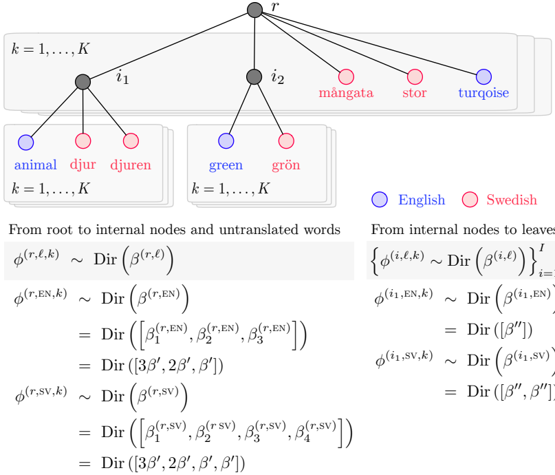
Figure 3 An illustration of the tree structure used in word-level models. Hyperparameters \beta^{(r,\ell)} and \beta^{(i,\ell)} are both vectors, and \beta' and \beta'' are scalars. In the figure, i_1 has three translations, so the corresponding hyperparameter \beta_1^{(r,\text{EN})} = \beta_1^{(r,\text{SV})} = 3\beta' .
