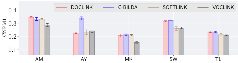
(a) score comparison of different models and languages with cardinality C = 10 .
