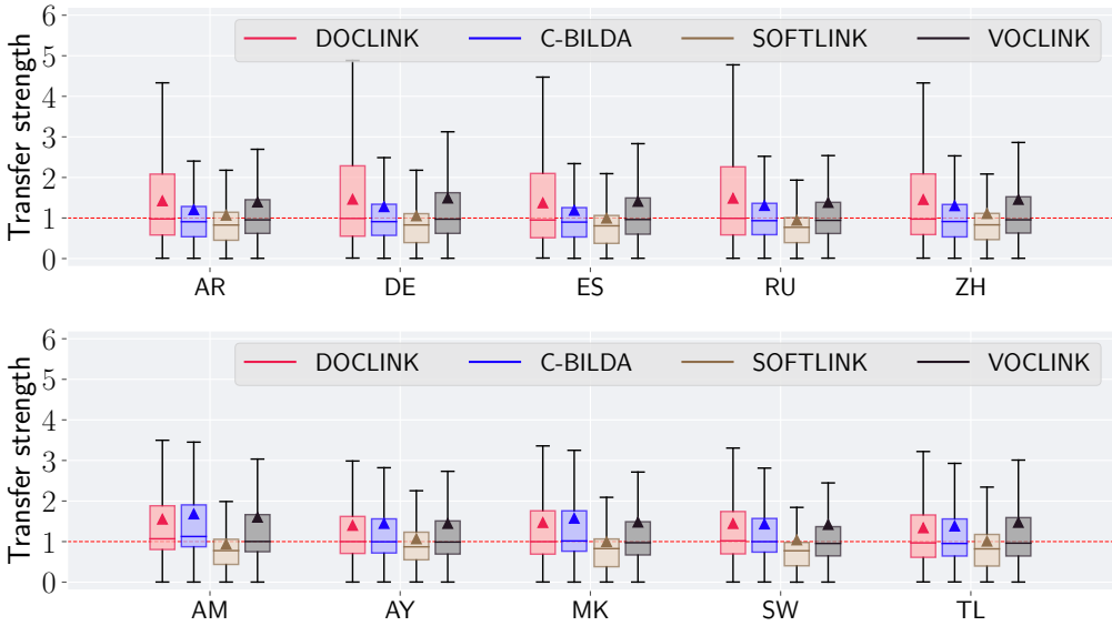
Figure 20 Comparisons of transfer strength. A value of one (shown in red dotted line) means an equal balance of transfer between document and word levels. We notice SOFTLINK has the most balanced transfer strength, whereas VOCLINK has stronger transfer at the document level although its transfer operation is defined on the word level.
