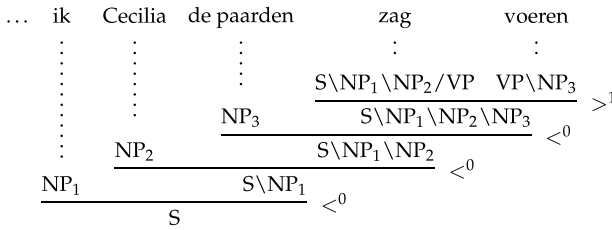
Figure 16 Straightforward derivation of Dutch cross-serial dependencies.
