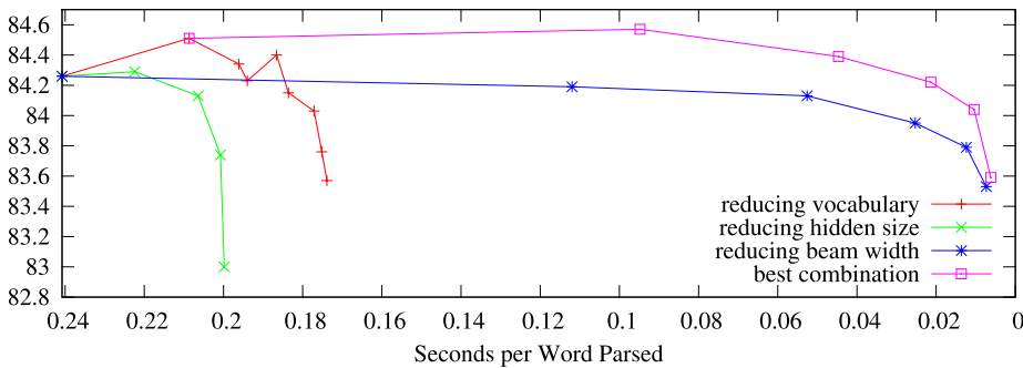
Figure 14 The parsing speed–accuracy trade-off when changing the meta-parameters of the model, on the English CoNLL-2009 development set. The vocabulary frequency threshold is increased from 5 to 10, 20, 30, 40, 60, 80, 120, and 160. The latent vector size is reduced from 80 to 70, 60, 50, and 40. The search beam width is reduced from 80 to 40, 20, 10, 5, and 3. The best combination keeps the vocabulary frequency threshold at 10 and reduces the search beam width as above.
