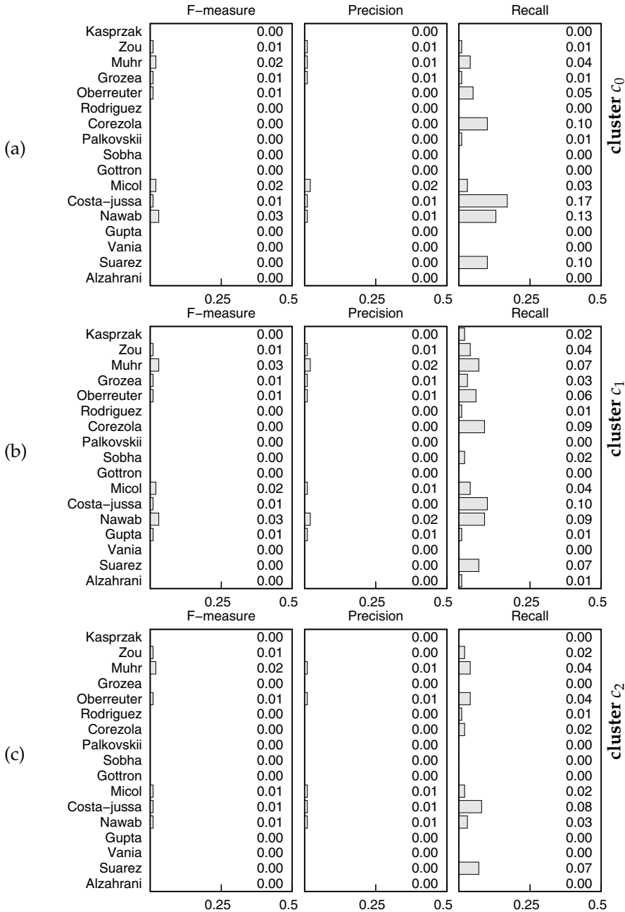
Figure 6 Evaluation of the Pan-10 competition participants' plagiarism detectors for (a) c_0 ; (b) c_1 ; and (c) c_2 .
