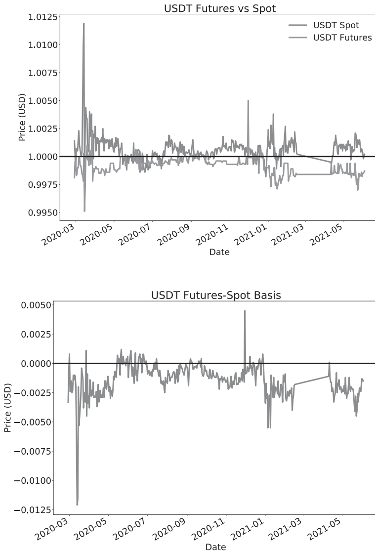
Figure 1. USDT spot and futures prices
