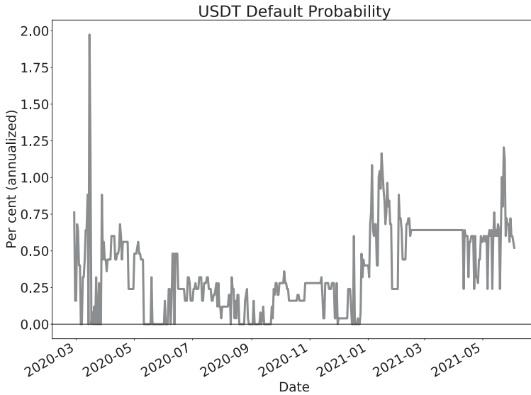
Figure 2. Estimate of probability of default P
