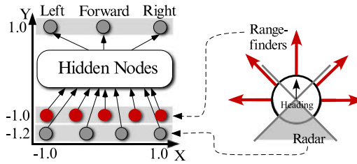
Figure 7. Substrate configuration and sensor layout. The controller substrate is shown at left. Whereas the number of hidden nodes for the fixed-substrate approach is determined in advance, ES-HyperNEAT decides on the positions and density of hidden nodes on its own. The sensor layout is shown on the right. The autonomous agent is equipped with five distance and four pie-slice sensors. Each rangefinder sensor indicates the distance to the closest obstacle in that direction. The pie-slice sensors act as a compass toward the goal (i.e., food), activating when a line from the goal to the center of the robot falls within the pie slice.
