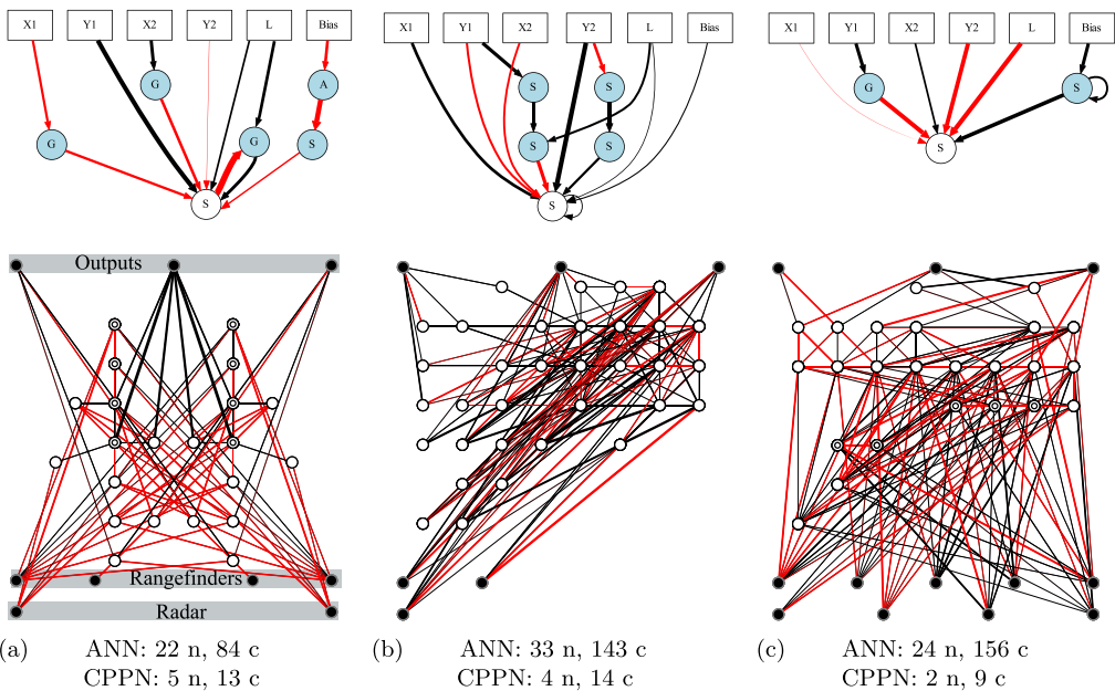
Figure 10. ES-HyperNEAT ANN solutions and their underlying CPPNs. Three ANN solutions (bottom) and the CPPNs (top) that encode them are shown together with the numbers of hidden neurons ( n ) and connections ( c ). ES-HyperNEAT evolves a variety of different ANNs, showing varying degrees of symmetry and network connectivity. In the electronic version, positive connections are dark (black), whereas negative connections are light (red). Line width corresponds to connection strength. Hidden nodes with self-recurrent connections are denoted by a smaller concentric circle. CPPN activation functions are denoted by G for Gaussian , S for sigmoid , and A for absolute value . The CPPNs receive the length L of the queried connection as an additional input.
